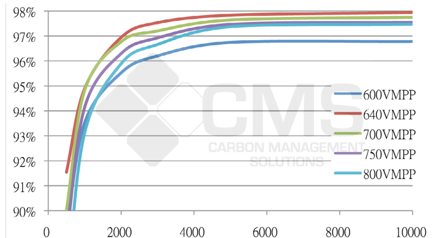
CMS - 10000SS Efficiency Chart
